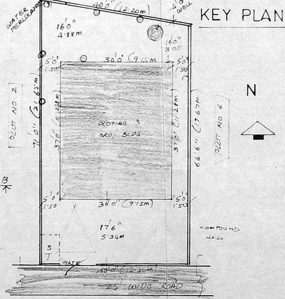
SITE PLAN
